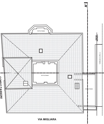
PIANTA PIANO COPERTURE
