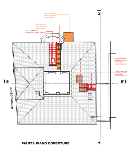
PIANTA PIANO COPERTURE
