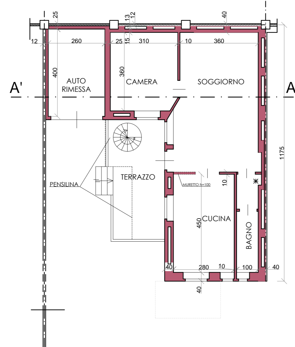
PIANO TERRENO
