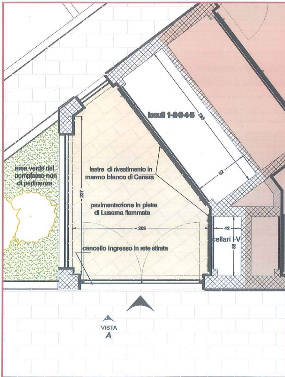
pianta TF3 -TF 7
